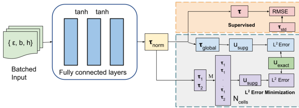
Figure 1: Schematic diagram of SPDE-Net
