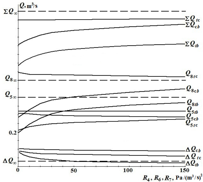
Figure 4: Air flow rates Q_5 , Q_8 , \Delta Q and \Sigma Q as functions of aerodynamic resistance for an elevator equipped with two bypass ducts (HC – lower and medium, CB – medium and upper, HB – lower and upper, \infty – no bypass ducts)
