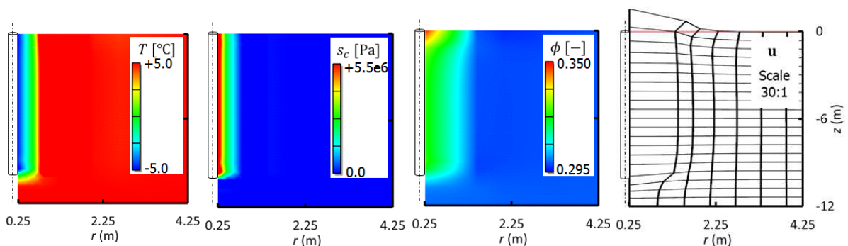
Fig.2 Temperature, cryosuction, porosity and deformation during freezing.
