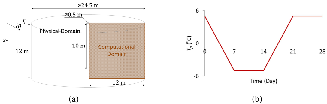
Fig.1 Energy pile: (a) geometry, (b) boundary condition – freezing/thawing cycle.
