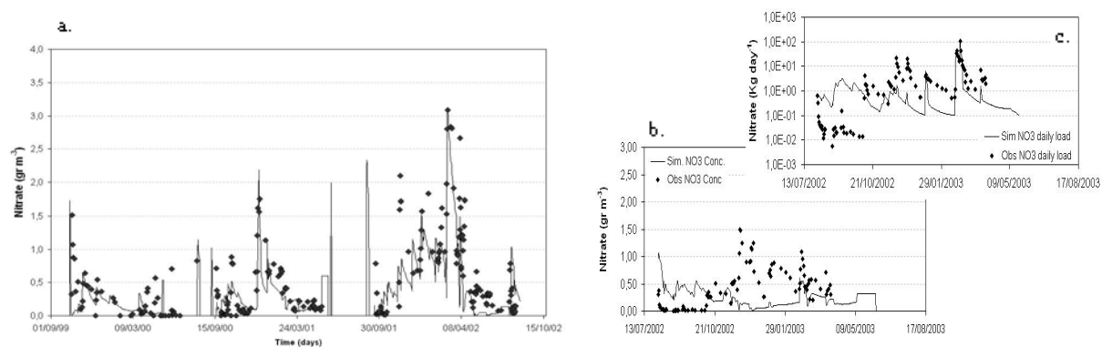
Figure 3. LU4-N model outputs (solid line) and observed nitrate concentration (black diamonds) a) for the three years calibration period (10/99-08/02); b) for the validation period (08/02-30/06); c) observed and simulated daily nitrate loads for the validation period (08/02-30/06).
