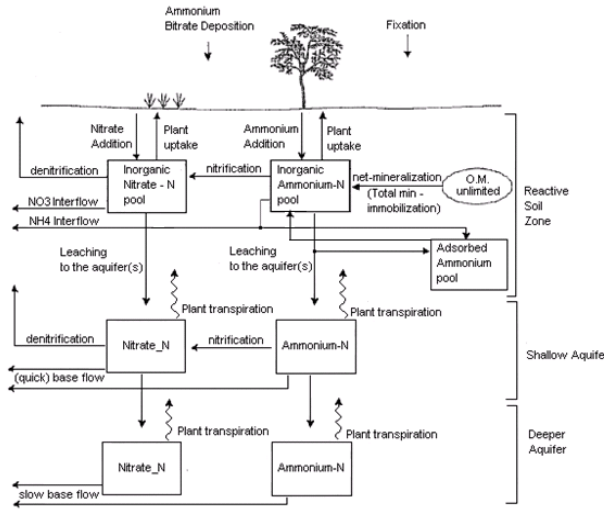
Figure 2. Nitrogen cycle in the soil and aquifers systems for the LU4-N model (modified form Whitehead et al. 1998)
