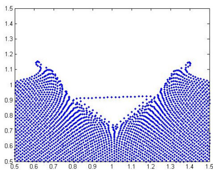
Figure 1 Water entry of a free falling wedge.
