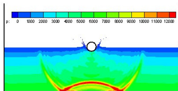
Figure 2 Water entry of a free falling sphere.
