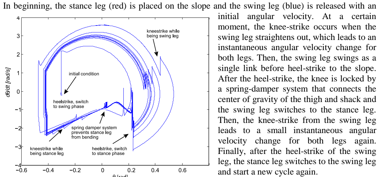
Figure 2. Phase portrait for the bipedal robot with multi-point contact foot
