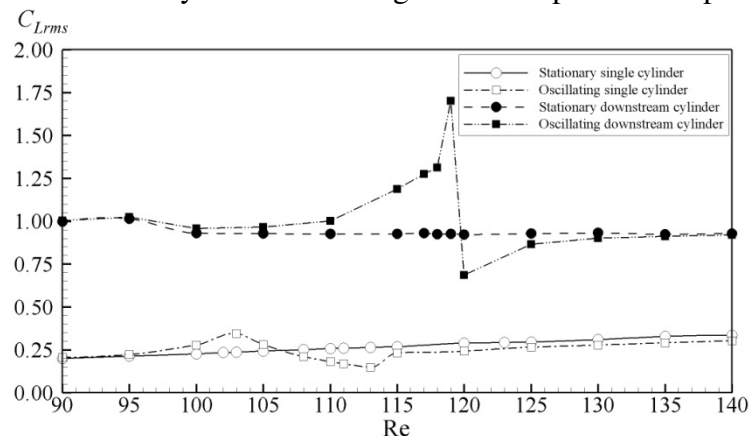
Figure 5: Root mean square of the lift coefficient versus Reynolds number for stationary and oscillating downstream cylinders in tandem arrangement and for fixed and oscillating single cylinders
