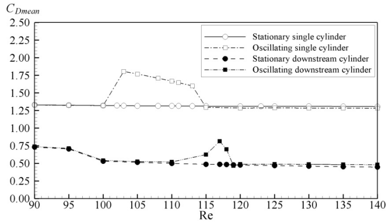
Figure 6: Mean drag coefficient versus Reynolds number for stationary and oscillating downstream cylinders in tandem arrangement and for fixed and oscillating single cylinders
