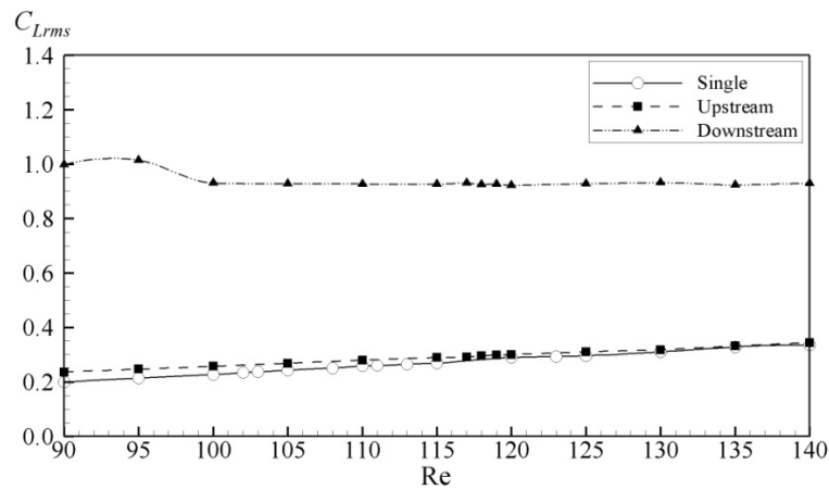
Figure 3: Root mean square of lift coefficient versus Reynolds number for stationary cylinders case
