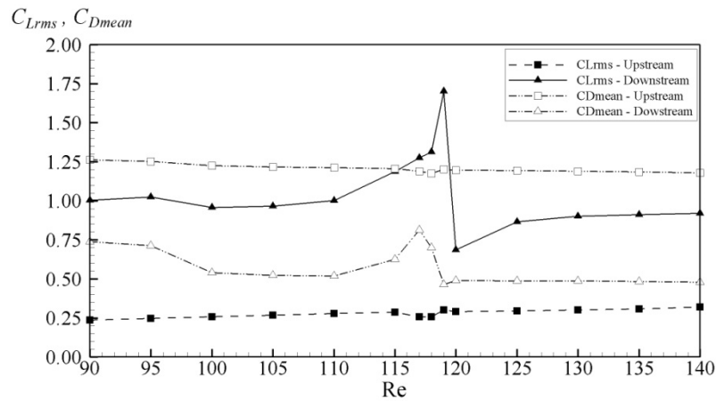
Figure 7: Root mean square of lift and mean drag coefficients versus Reynolds number for stationary upstream and oscillating downstream cylinders in tandem arrangement
