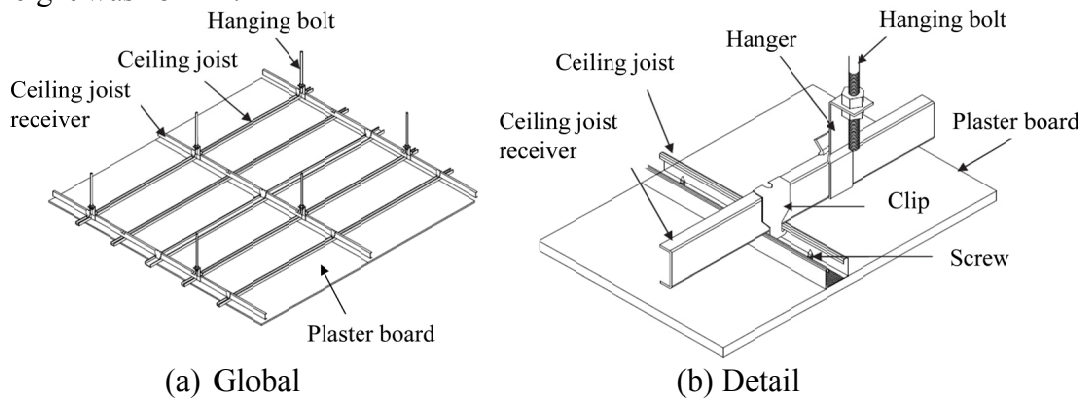
(a) Global (b) Detail Figure 3: Typical configuration of suspended ceiling (perspective)
