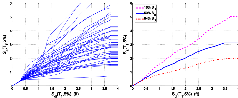
Figure 4: Complete set of 44 IDA curves and the summary 16 th , 50 th , 84 th percentile IDA curves in S_a - S_{di} coordinates as produced by nonlinear response history analysis for the equivalent single-degree-of-freedom fitted to a 4-story reinforced concrete moment frame building model.
