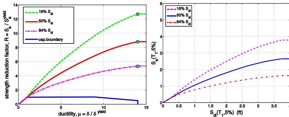
Figure 5: Percentile IDA curves in R - \mu and S_a - S_{di} coordinates as produced by SPO2IDA [14] for the equivalent single-degree-of-freedom fitted to a 4-story reinforced concrete moment frame building model.
