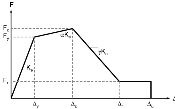
Figure 6: The backbone characteristics used in the FEMA 440A equation for maximum strength factor, R_{di} , to avoid dynamic instability.
