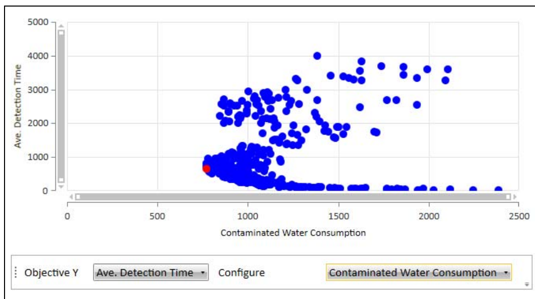
Figure 2. Average detection time vs contaminated water consumption
